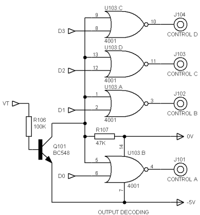
OUTPUT DECODING
