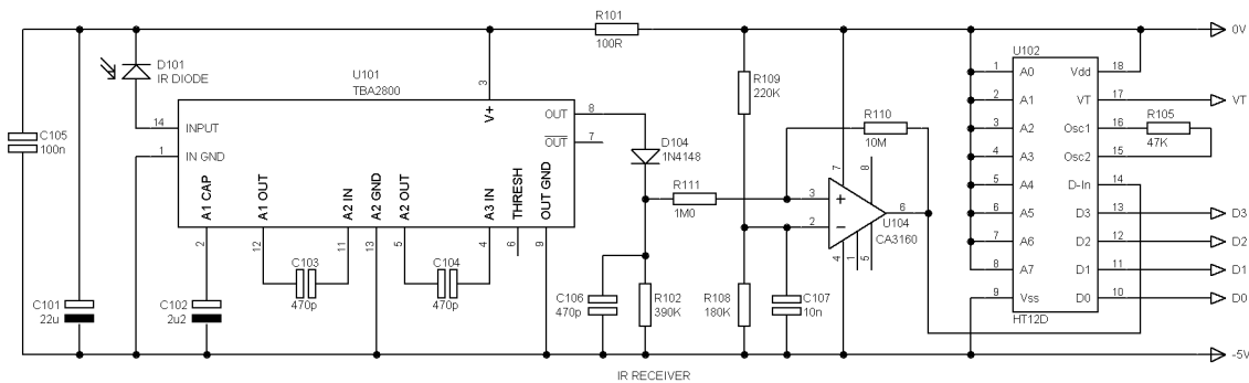
IR RECEIVER
